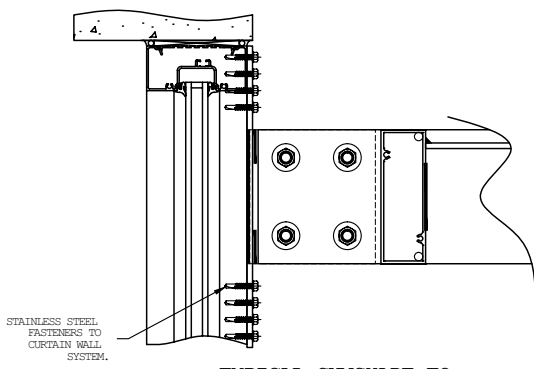
TYPICAL SUNSHADE TO CURTAIN WALL INSTALLATION
