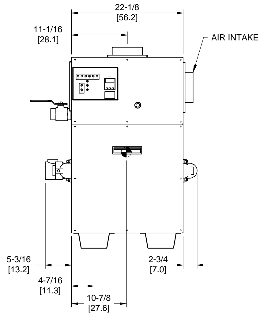
FRONT VIEW
