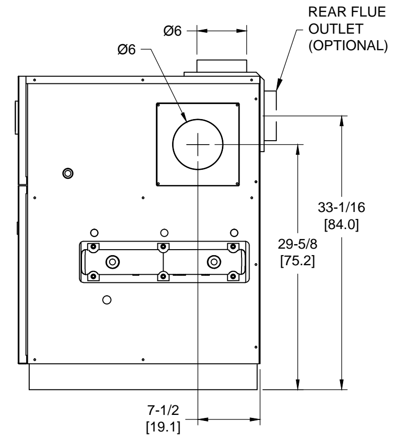
RIGHT VIEW
