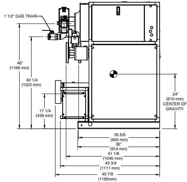
LEFT VIEW
