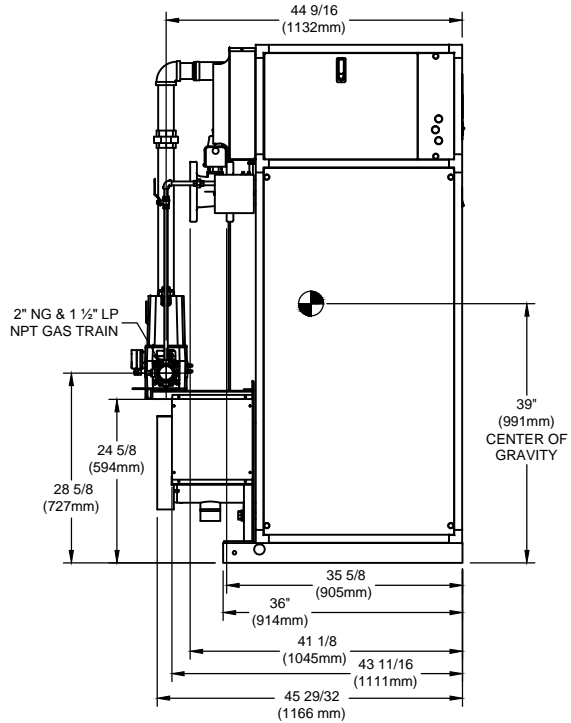
LEFT VIEW
