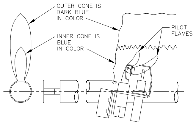
Figure 3 - Pilot and Main Burner Flames
